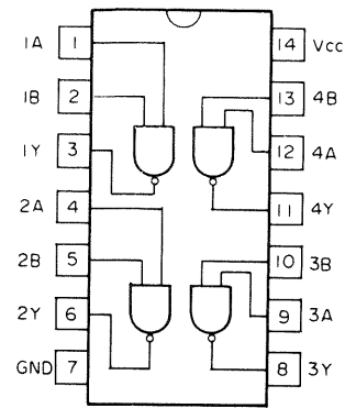
SN74ALS00AN
