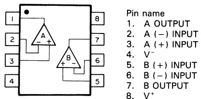
NJM072M
