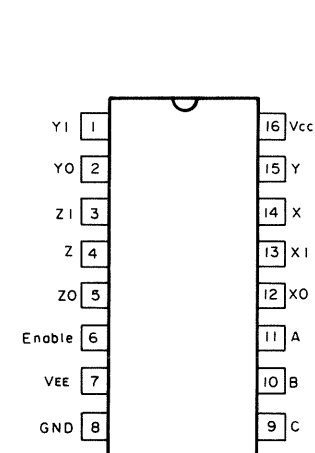
MC74HC4053N
