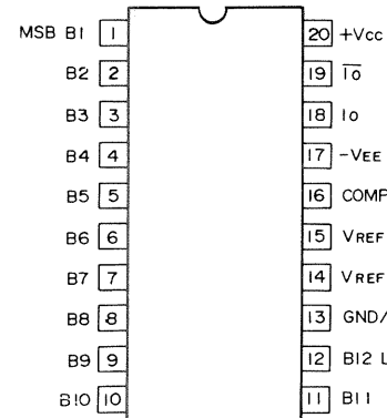
AM6012DC
