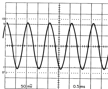
Fig. 14 DC +4.8V
