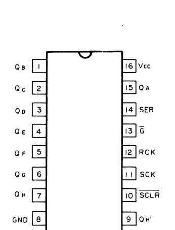
HD74HC595P
