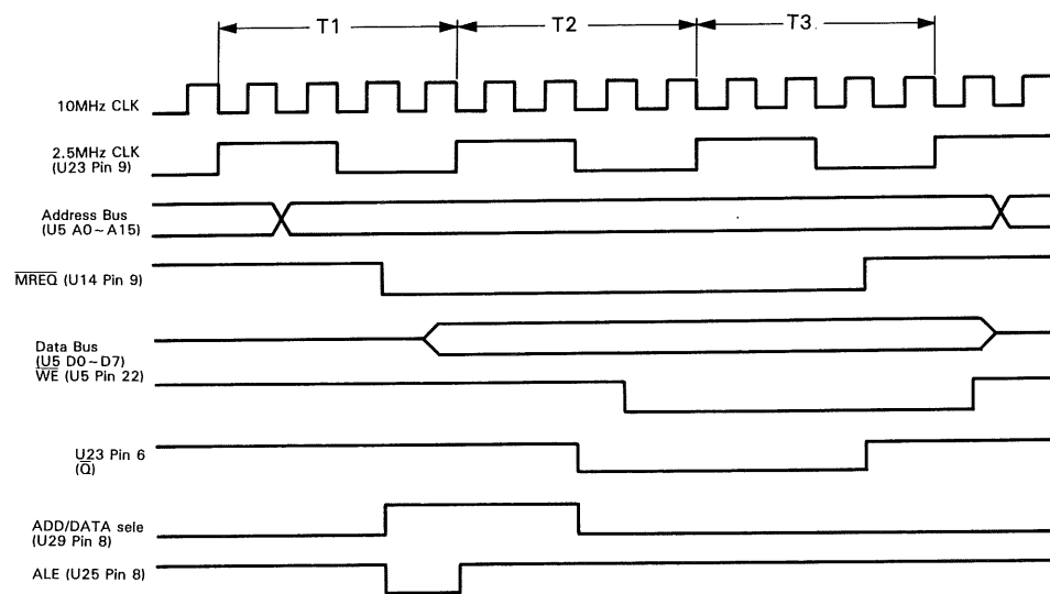
Address/Data Select Timing Chart (X77-1490-00)
