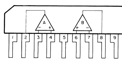
NJM4556S
