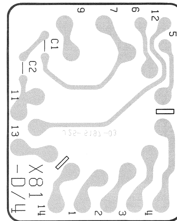
CRT SOCKET
