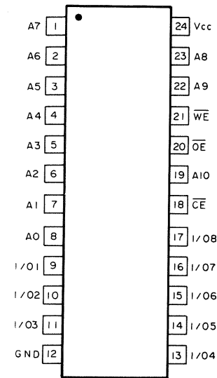
LC3517BML-15
