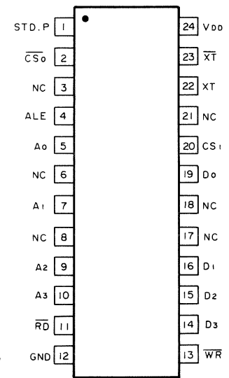
MSM6242BGS-VK
