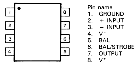
NJM311M
