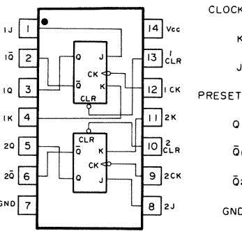
HD74LS107AFP HD74HC107FP
