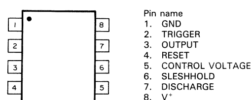
NJM555M
