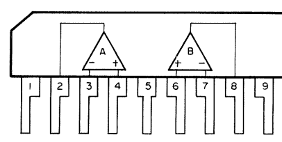
NJM072S
