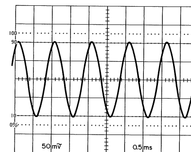
Fig. 15 DC +4.8V
