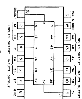
HD74LS157FP
