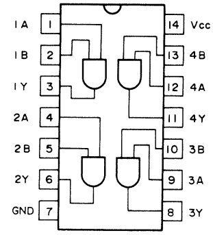
SN74ALS08N HD74HC08FP
