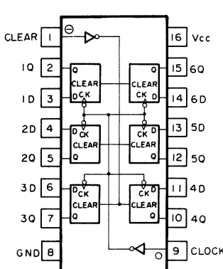
HD74HC174FP
