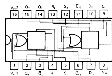
MC10H131L
