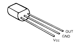
PST518B
