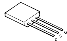
2SK241 (GR)
