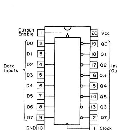
HD74HC564FP
