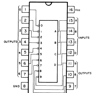
HD74LS42P
