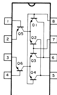
μPA101G
