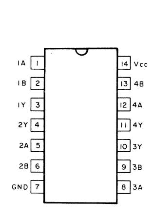
HD74HC7266FP
